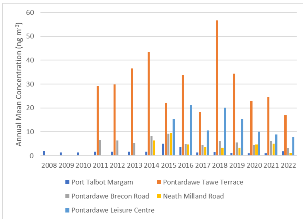
Figure 2-4 Trend in Annual Mean Concentrations of Nickel 2008 - 2022
